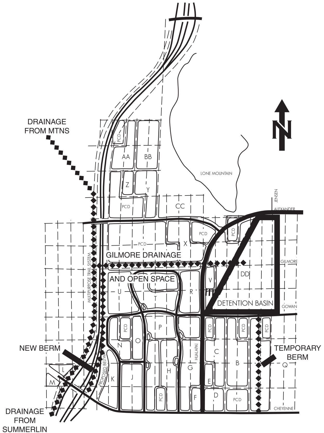
Figure 16 – DRAINAGE MASTER PLAN
