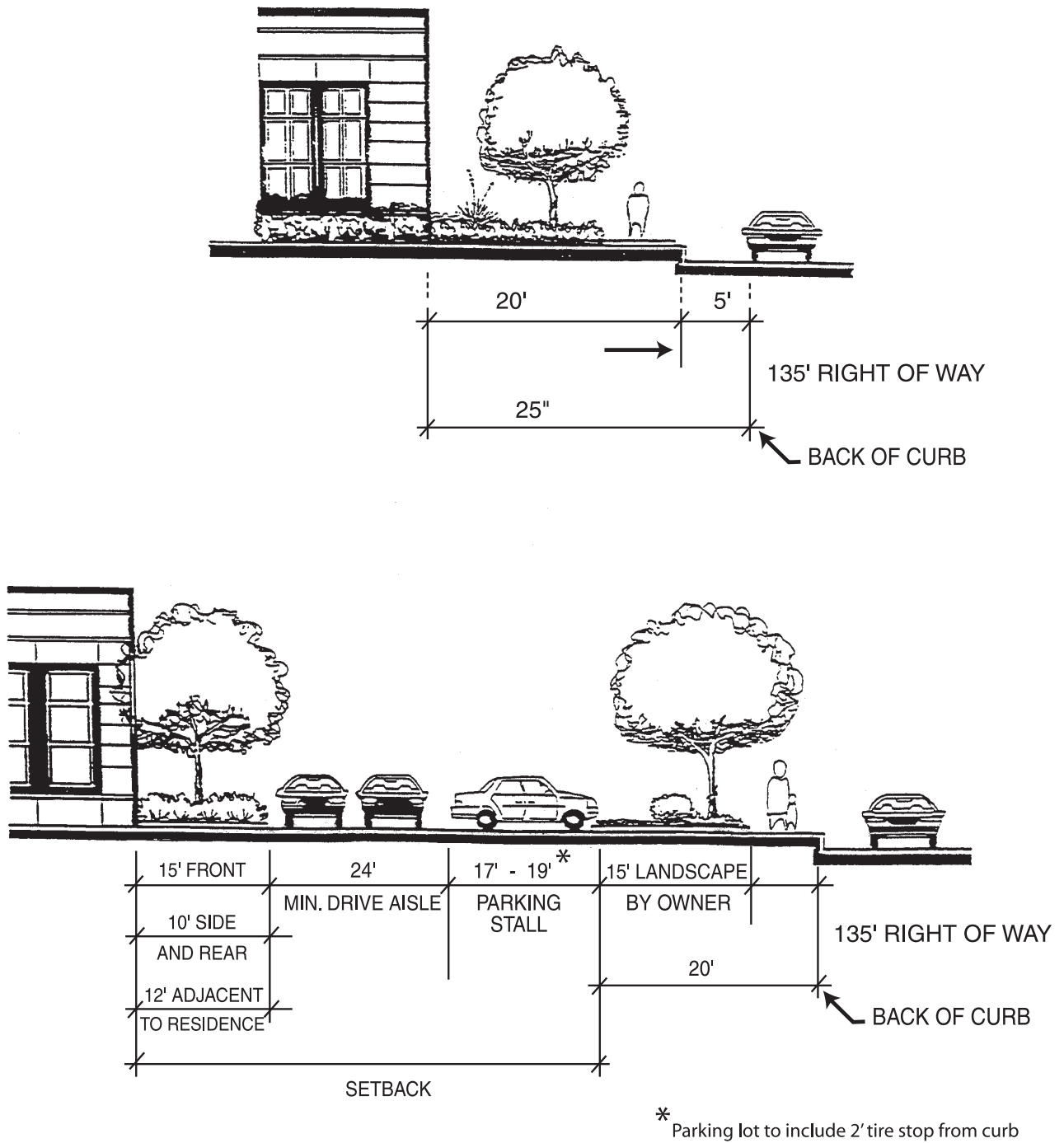
Figure 12 – VEHICULAR AND BUILDING SETBACKS, BUILDING HEIGHTS NEIGHBORHOOD OR VILLAGE COMMERCIAL 135' right of way
