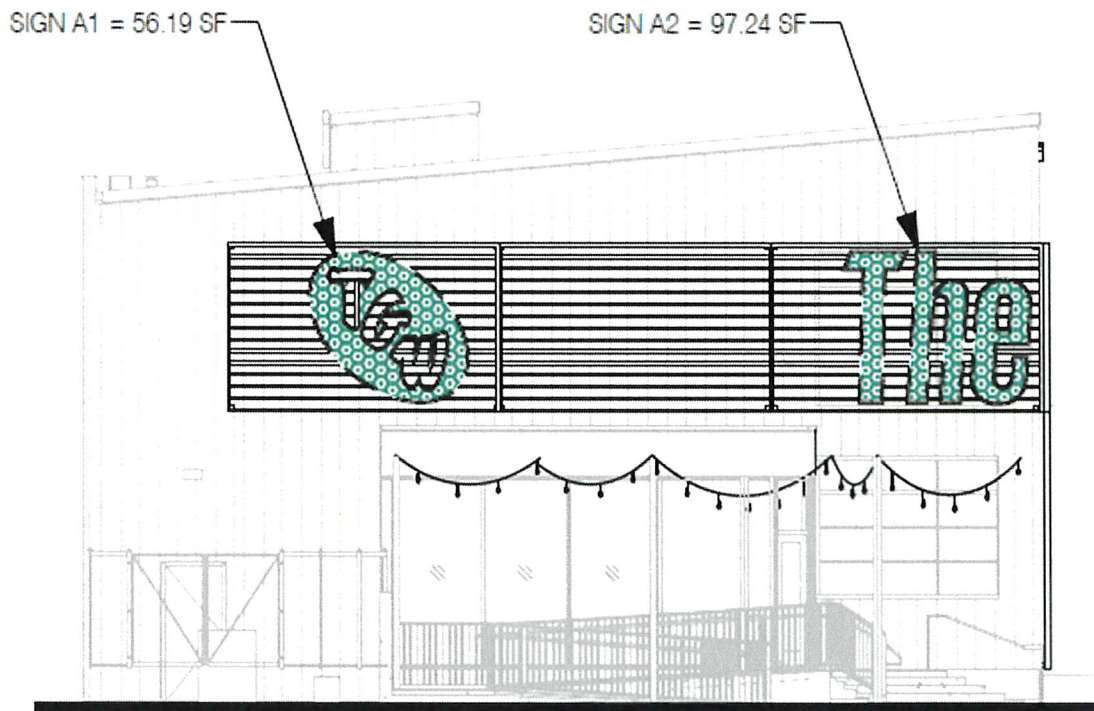
NORTH ELEVATION SCALE: 1/16" = 12"
