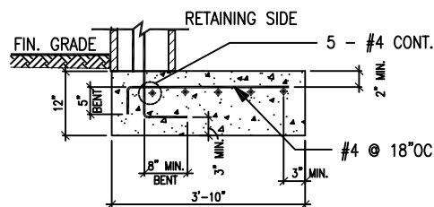
OPTIONAL FOOTING FOR 2' RETAINING WALL
