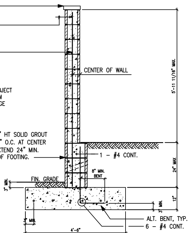
2' RETAINING WALL
