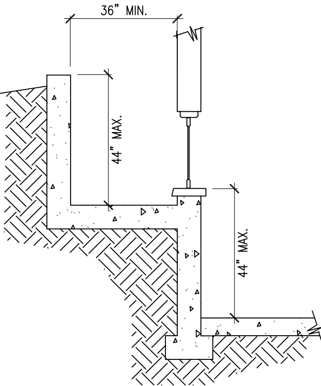
CROSS SECTION
