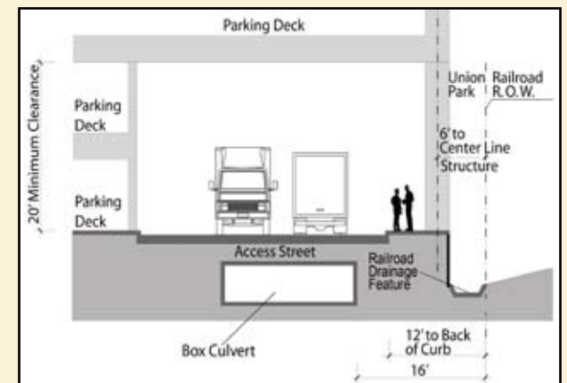
Typical Service Access Section (Along Railroad) Note: Subject to change depending on engineering design
